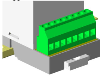
5 / 5.08 mm pitch Terminal Max. 16 ( 8 x 2 )
