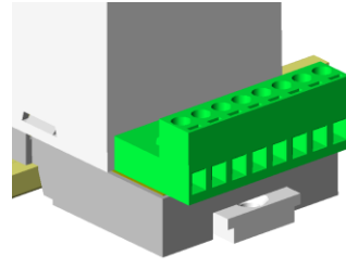
5 / 5.08 mm pitch Plug-In Terminal: Max. 16 ( 8 x 2 )
